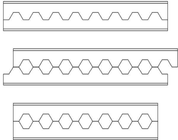
Fig 1: Castellated Beam
