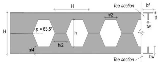
Fig. 2: Tee- section
