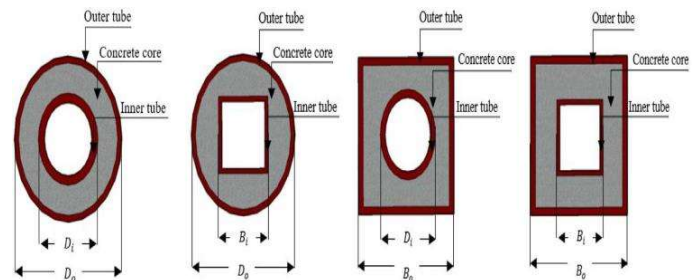
Fig-1: Different configuration of CFDST column
